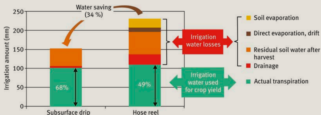
5 Simulation of irrigation water amounts transpired by the crop or lost for corn with subsurface drip (SSD) or sprinkler irrigation (hose reel machine).
